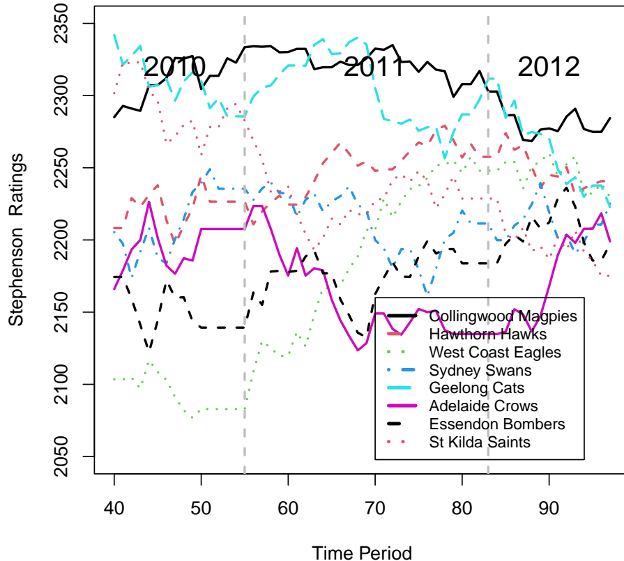
Figure 2: Plots of ratings traces for eight football teams from mid-2010 to mid-2012.
