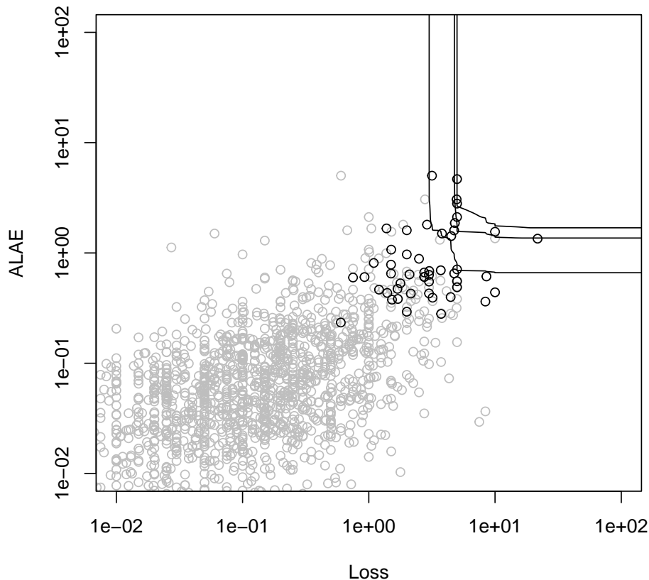
Figure 4: Estimated quantile curves Q(\hat{F}, p) for p = 0.98, 0.99, 0.995 based on the componentwise block maxima data shown as black circles, using the Capéraa-Fougères-Genest nonparametric estimate of the dependence function and using empirical marginal estimation.
